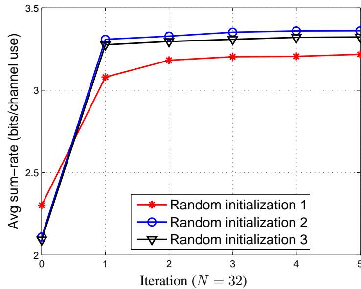
Figure 3.11: Average sum-rate vs. iterations for solving joint pairing and power allocation problem P0 , (iterative pairing algorithm and without direct link)
